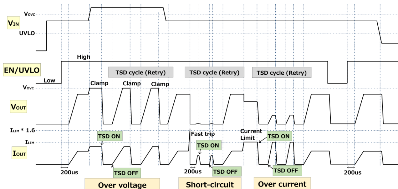
Timing chart (auto-retry type)
