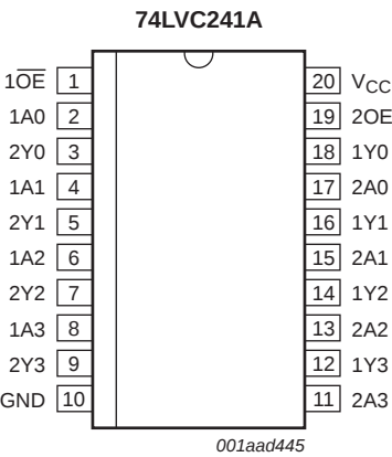
Fig 4. Pin configuration for SO20 and (T)SSOP20
