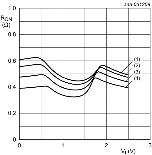
Fig. 8. ON resistance as a function of input voltage; V_{CC} = 1.5\text{ V}
