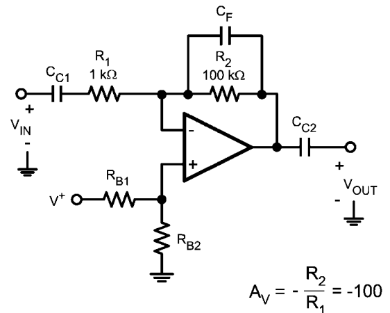
FIGURE 4. High Gain Inverting Amplifier
