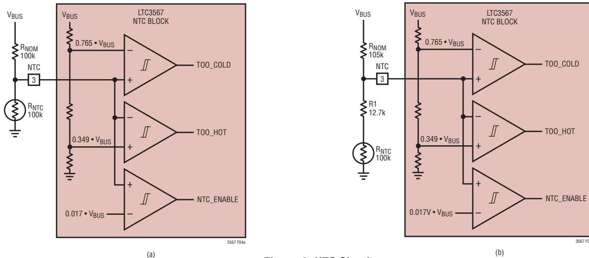
Figure 4. NTC Circuits
