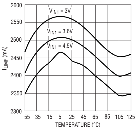
Buck-Boost Regulator Current Limit vs Temperature
