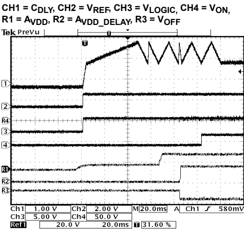
FIGURE 10. START-UP SEQUENCE
