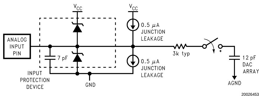
FIGURE 22. A/D Pin Model (Single Ended Mode)
