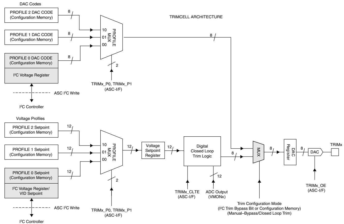
Figure 26. TrimCell Architecture
