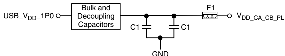
Figure 53. USB\_V_{DD\_1P0} Power Supply Filter Circuit
