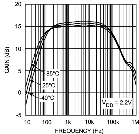
FIGURE 5. LMV1012-15 Gain vs. Frequency Over Temperature
