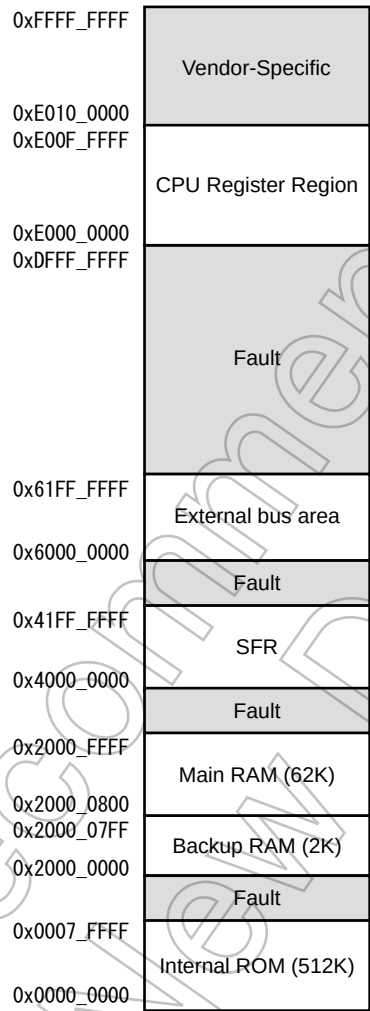
Figure 5-1 Memory Map (TMPM366FD)
