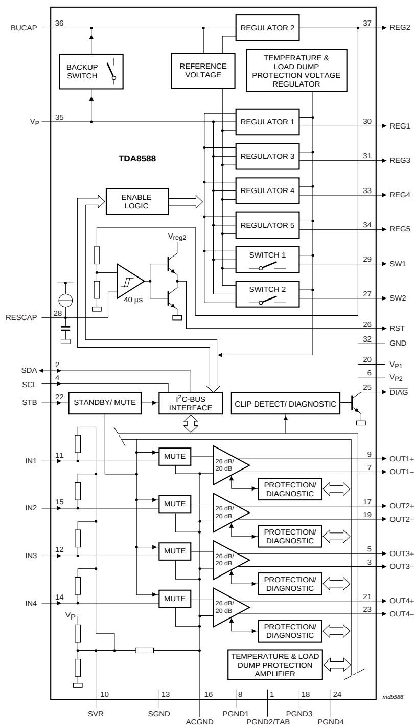
Fig.1 Block diagram.
