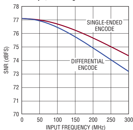
SNR vs Input Frequency, -1dBFS, 20MSPS, 2V Range
