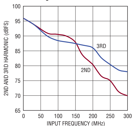
2nd, 3rd Harmonic vs Input Frequency, -1dBFS, 20MSPS, 2V Range
