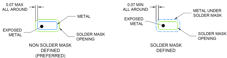
LAND PATTERN EXAMPLE EXPOSED METAL SHOWN SCALE: 20X
