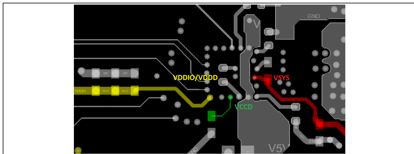
Figure 18 Bottom layer connection for V DDIO , V DDP , V SYS and V CCD
