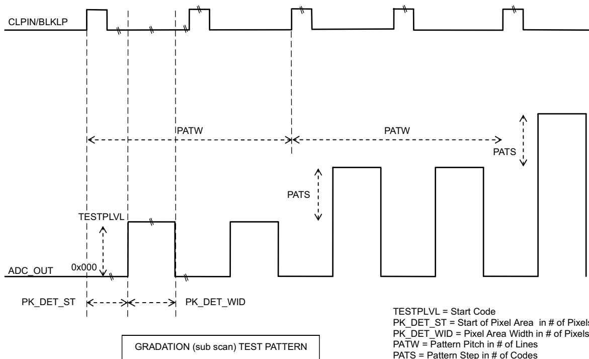
Figure 31. Gradation (Sub Scan) Test Pattern
