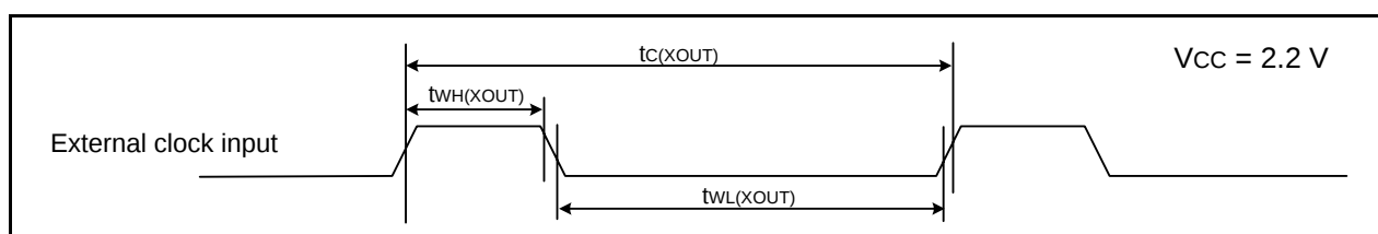
Figure 5.44 External Clock Input Timing Diagram when V_{CC} = 2.2\text{ V}
