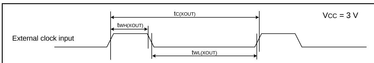
Figure 5.15 External Clock Input Timing Diagram when V_{CC} = 3\text{ V}
