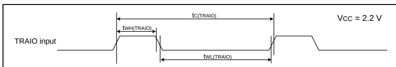
Figure 5.45 TRAIO Input Timing Diagram when V_{CC} = 2.2\text{ V}
