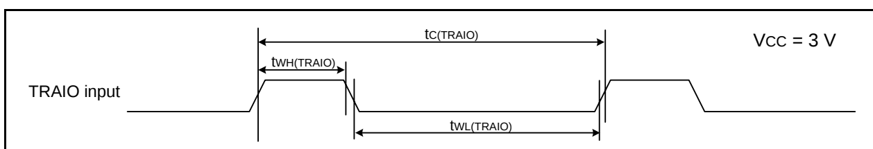
Figure 5.16 TRAIO Input Timing Diagram when V_{CC} = 3\text{ V}
