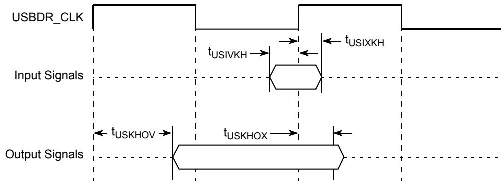
Figure 29. USB Signals
