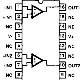
HA-5142 (SOIC)
