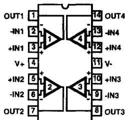
HA-5144 (PDIP, Cerdip)
