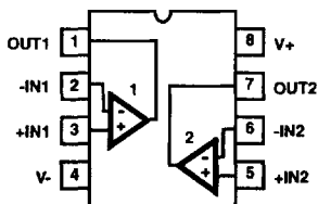
HA-5142 (PDIP, Cerdip)
