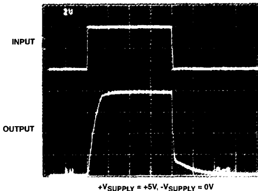
LARGE SIGNAL RESPONSE
