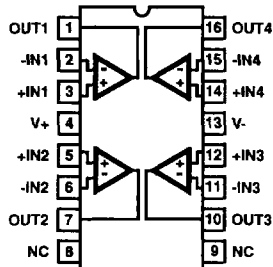
HA-5144 (SOIC)
