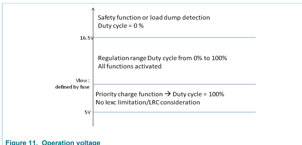
Figure 11. Operation voltage
