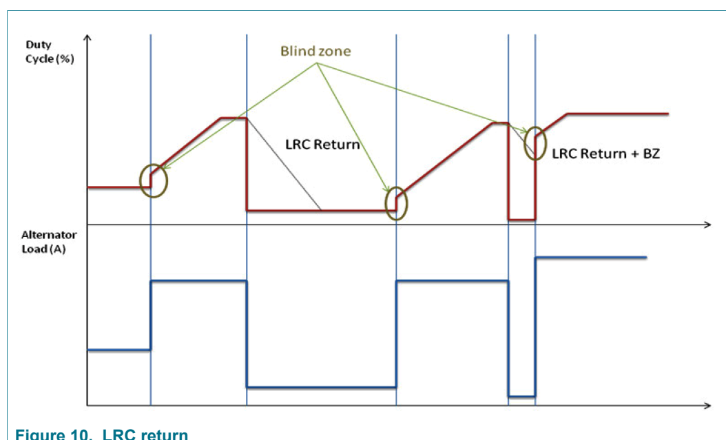
Figure 10. LRC return
