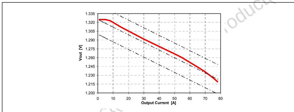
Figure 27. Load Regulation.
