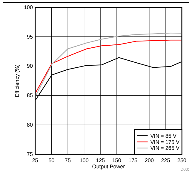
Figure 13. Efficiency vs Output Power
