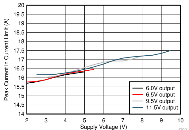
Figure 7-1. Peak Inductor Current vs Supply Voltage ( F_{SW} = 440 \text{ kHz} , R_S = 7 \text{ m}\Omega , R_F = 100 \text{ }\Omega , C_F = 2.2 \text{ nF} )
