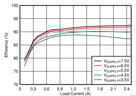
Efficiency ( V_{\text{LOAD}} = 9.5 \text{ V} , F_{\text{SW}} = 440 \text{ kHz} )
