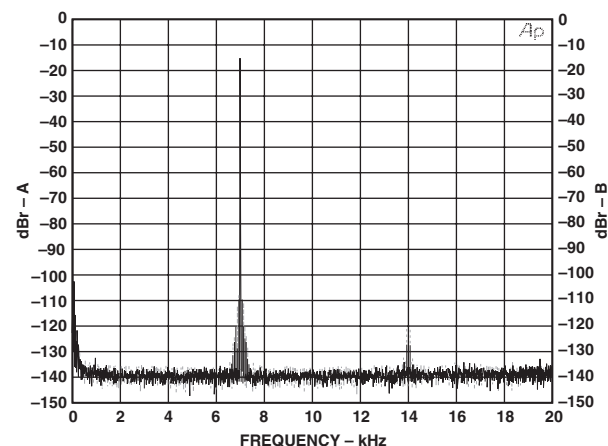
Figure 19. Two-Tone Test
