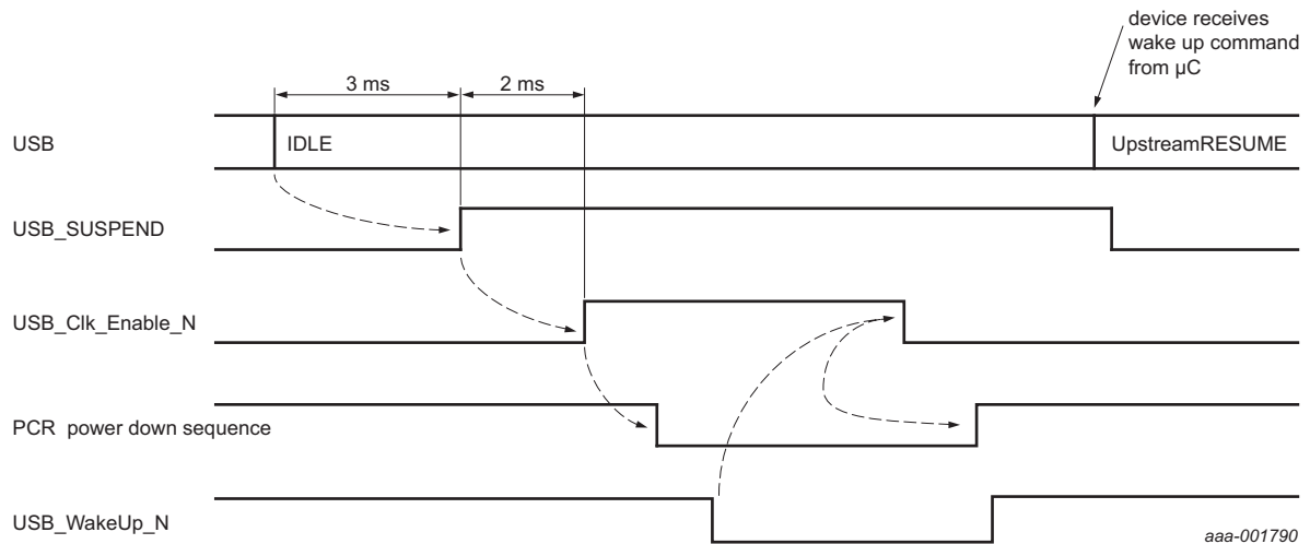
Fig 16. RemoteWakeUp by uC
