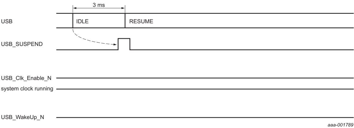
Fig 15. Resume by host / clocks running
