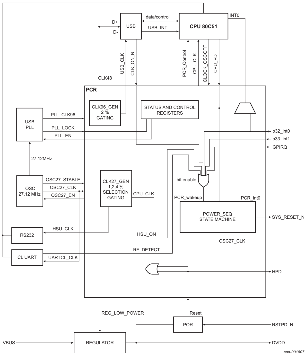
Fig 33. PR533 Power Management block diagram
