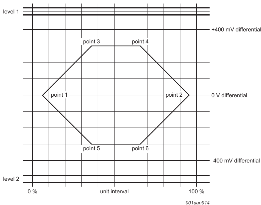
Fig 54. Transmit waveform at DP/DM
