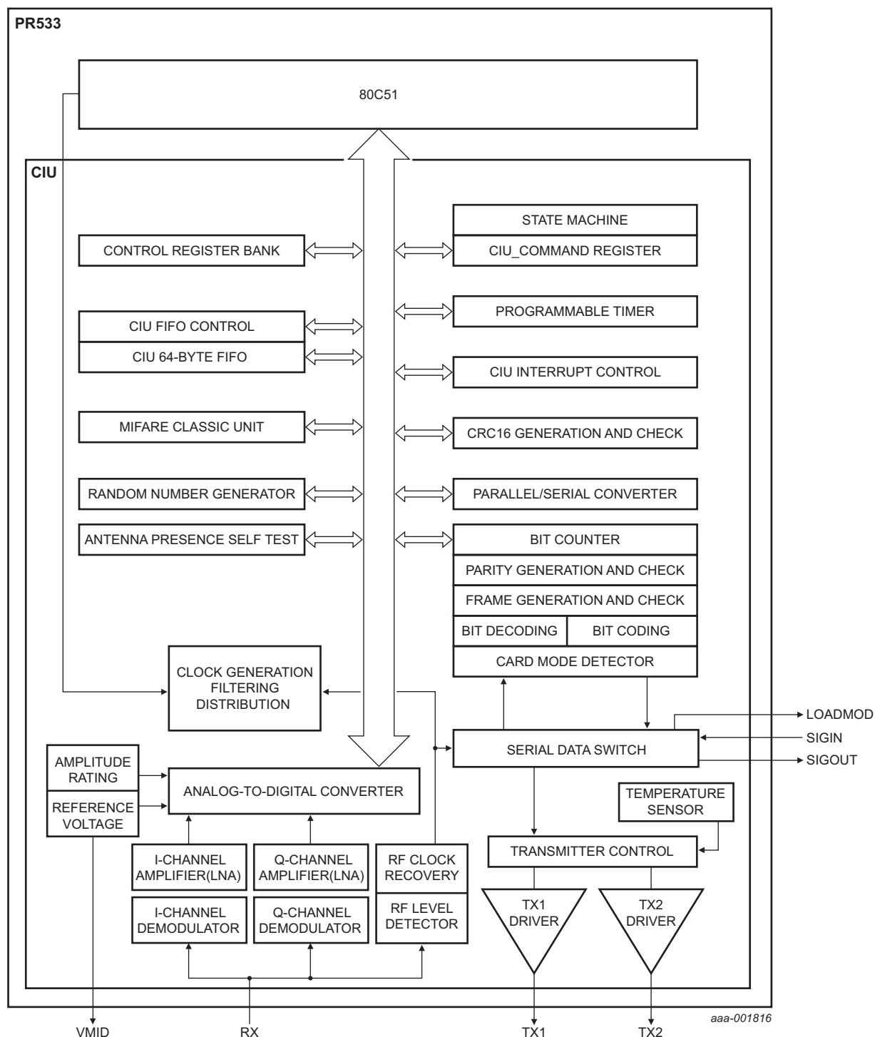
Fig 42. CIU detailed block diagram
