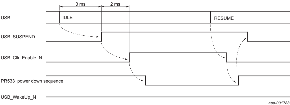
Fig 14. Resume by host/clocks stopped
