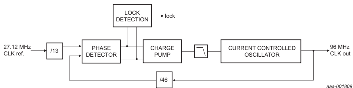
Fig 35. USB PLL
