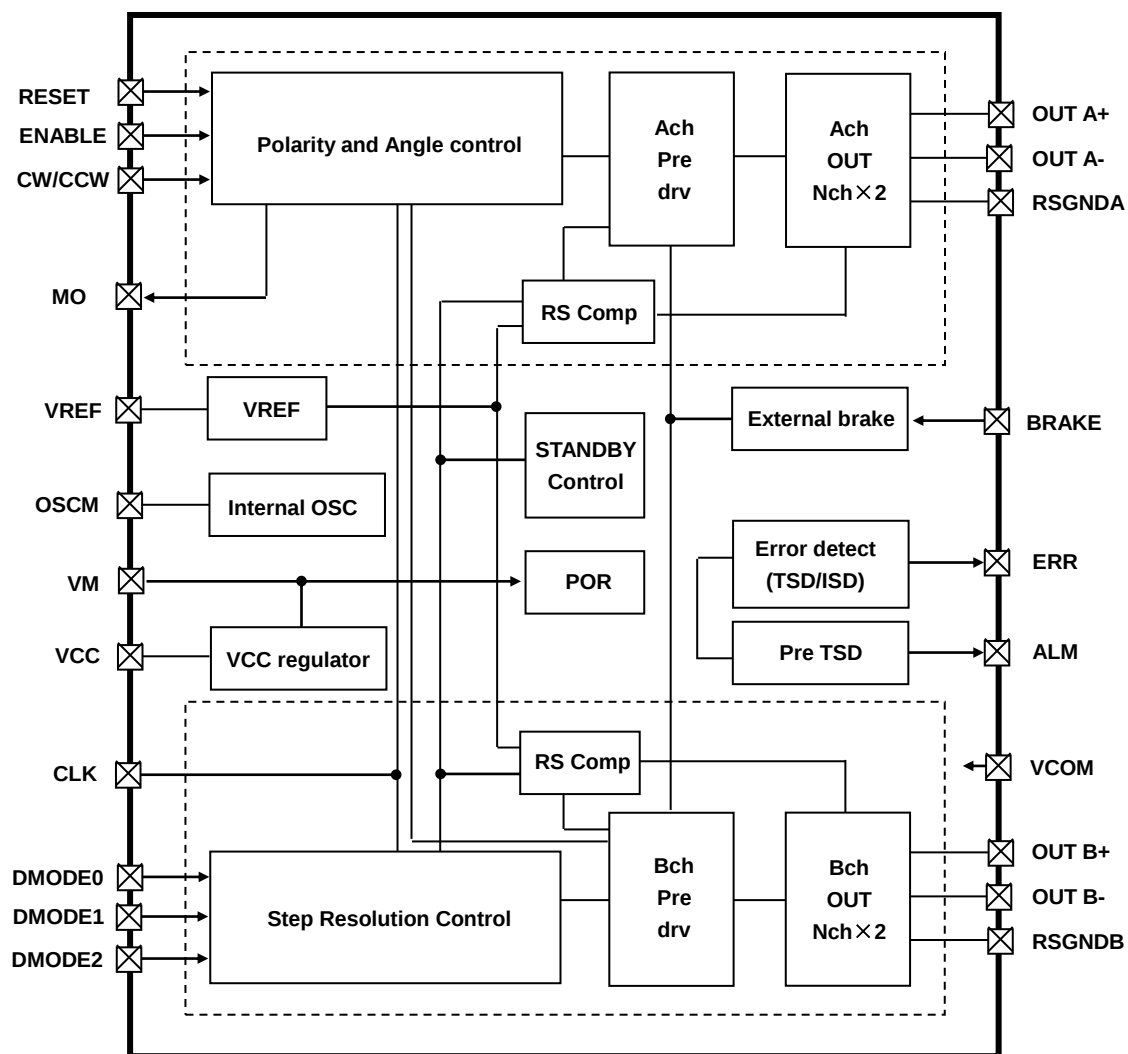
TB67S149AFTG block diagram
