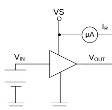
Test Setup 8 Clamp Diode Leakage Current
