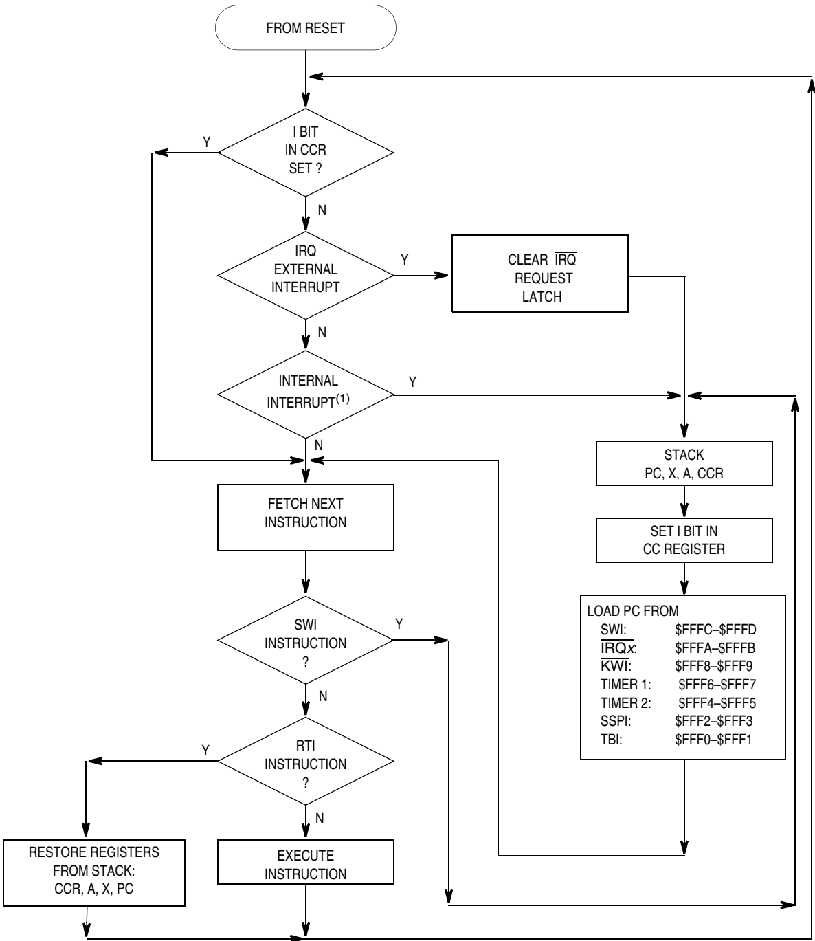
Figure 4-4. Interrupt Flowchart
