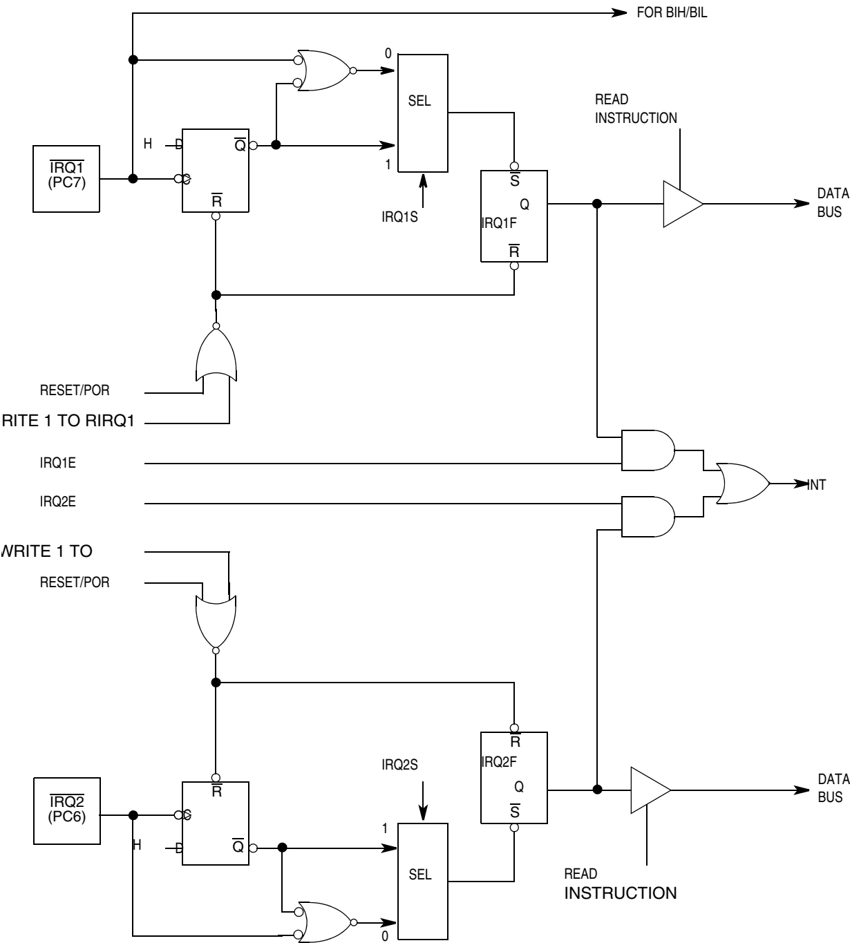
Figure 4-5. \overline{\text{IRQ1}} and \overline{\text{IRQ2}} Block Diagram
