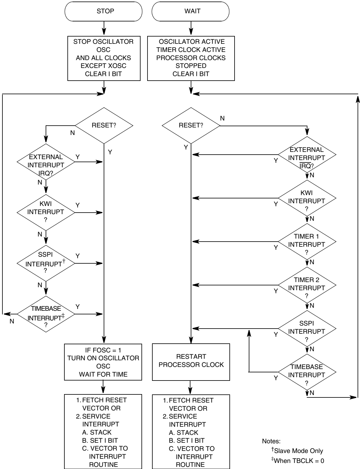
Figure 5-2. Stop/Wait Flowcharts
