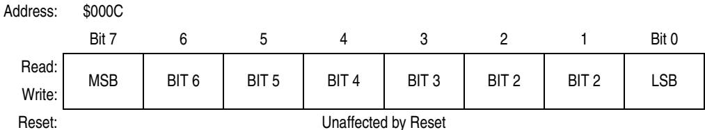
Figure 8-6. Serial Peripheral Data Register (SPDR)
