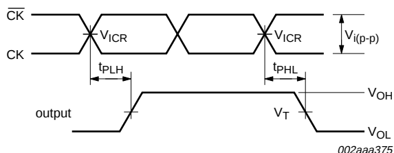
Fig 12. Voltage waveforms; propagation delay times (clock to output)
