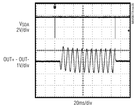
SOFTWARE SHUTDOWN ON- AND OFF-RESPONSE
