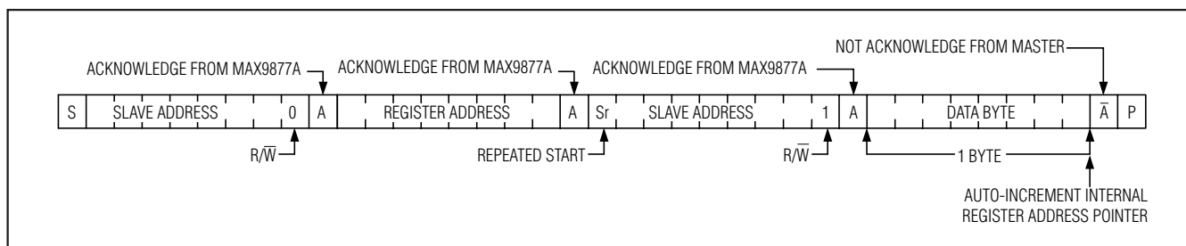
Figure 11. Reading One Indexed Byte of Data from the MAX9877A
