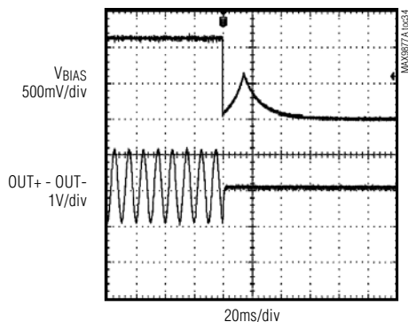
HARDWARE SHUTDOWN RESPONSE
