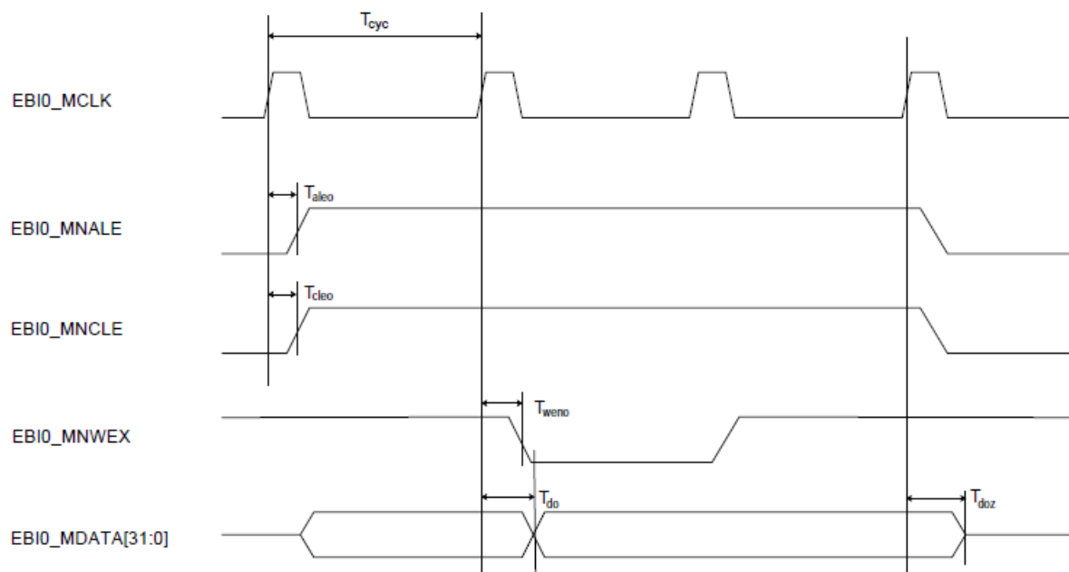
Figure 19. NAND Flash Write Timing
