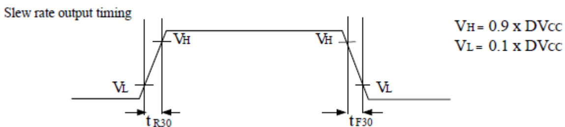
Figure 10. Slew Rate High Current Output Timing
