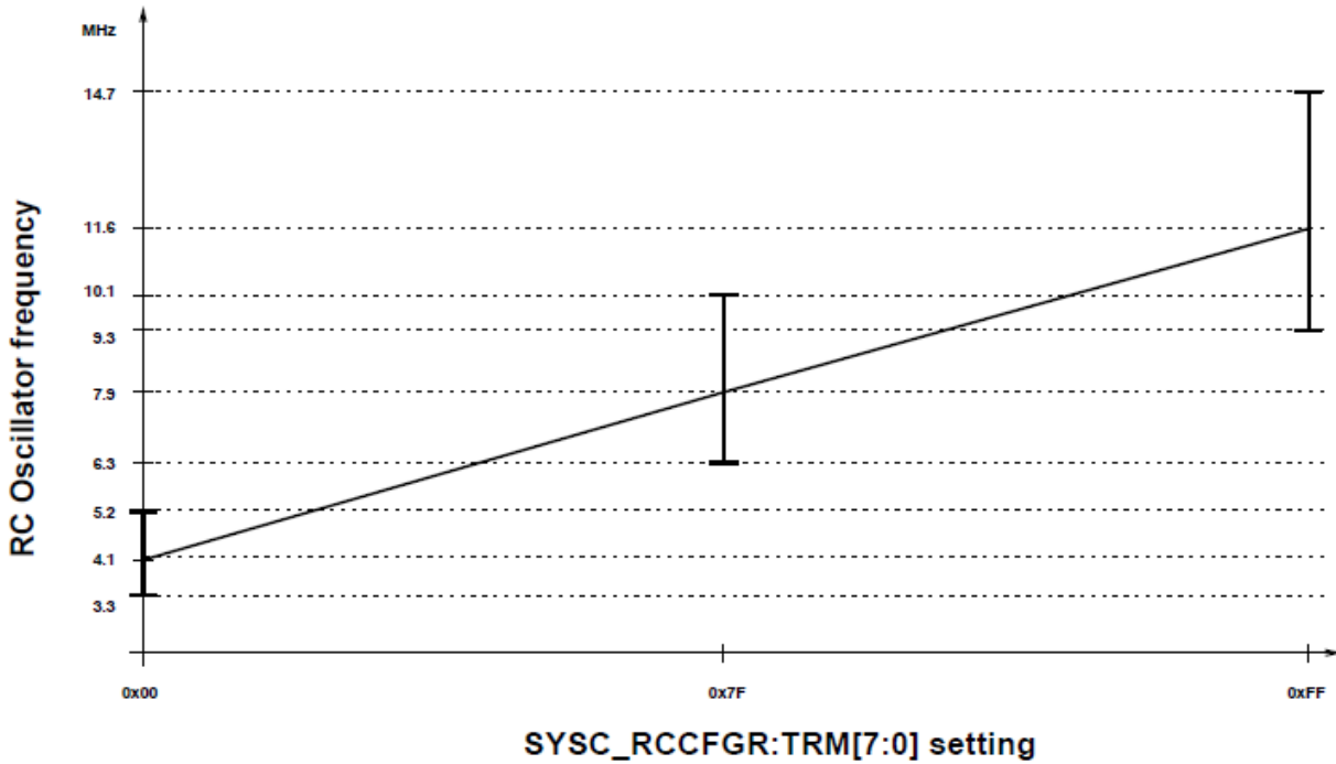
Figure 21. RC Oscillator Frequency at SYSC_RCCFGR:SFREQ = 0
