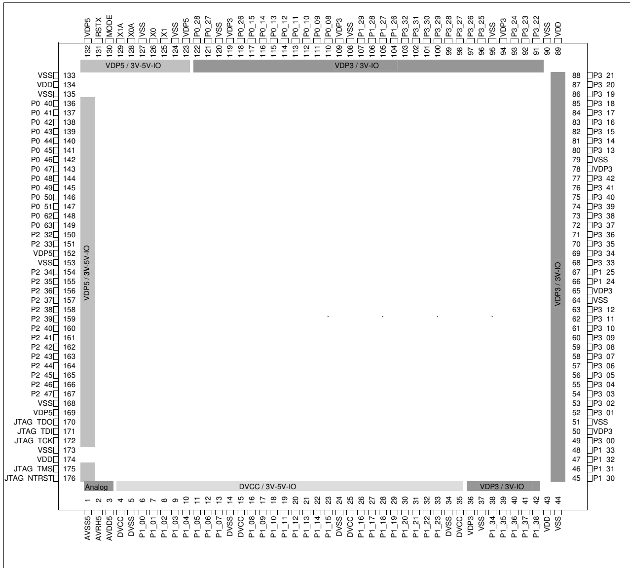
Figure 1. QFP-176 Pin Assignment
