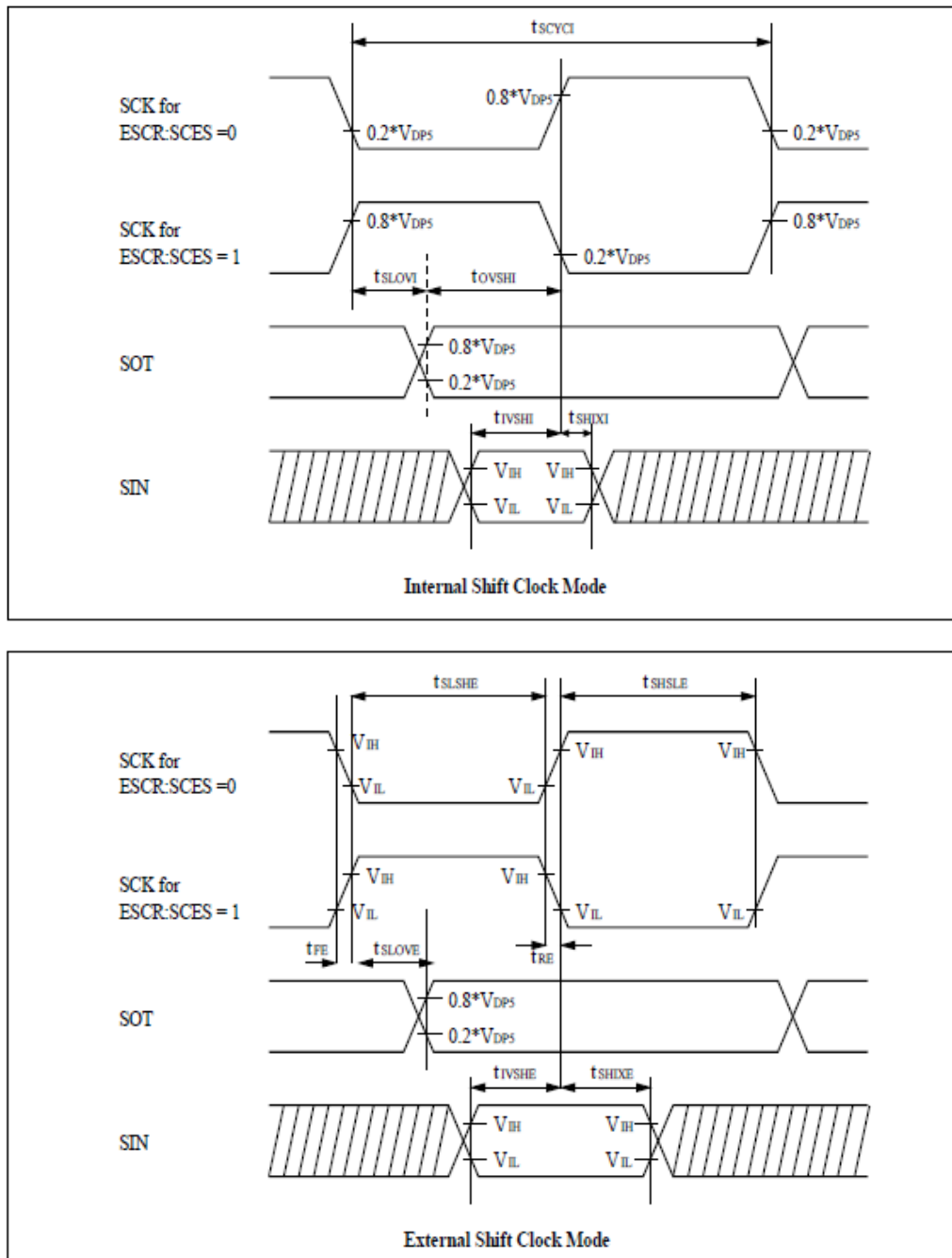
Figure 11. USART Timing
