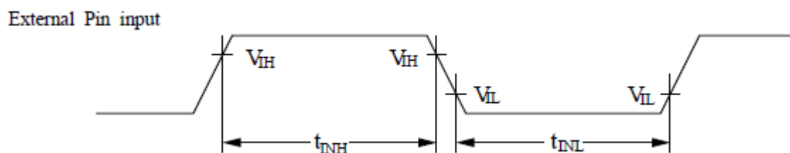
Figure 9. External Input Timing
