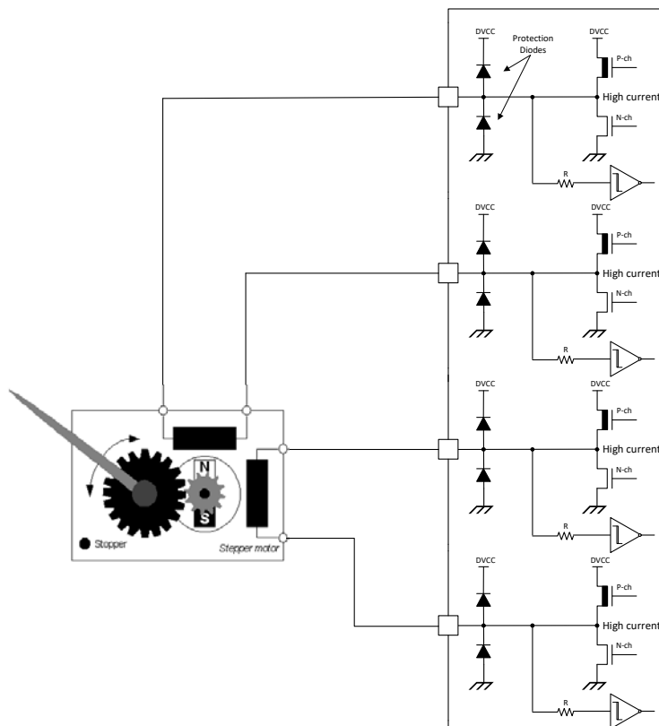
Figure 6. ESD Protection Structure for SMC Pins
