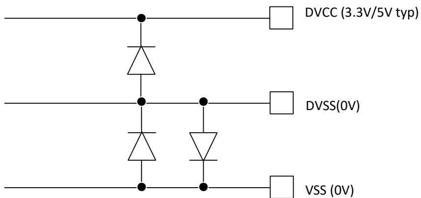
Figure 27. ESD Diodes between DVCC, DVSS and VSS
