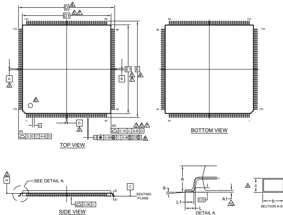
Figure 2. QFP-176 Package Dimensions
