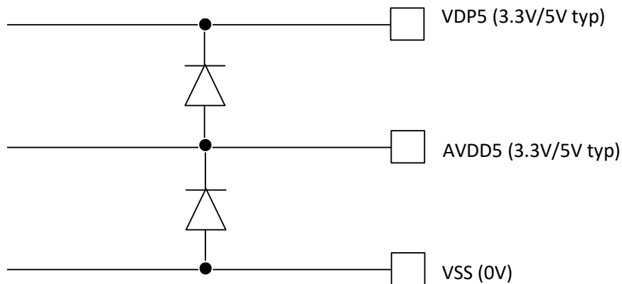
Figure 28. ESD Diodes between VDP5, AVDD5 and VSS
