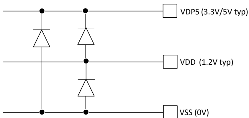
Figure 24. ESD Diodes between VDP5, VDD and VSS
