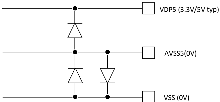
Figure 25. ESD Diodes between VDP5, AVSS5 and VSS
