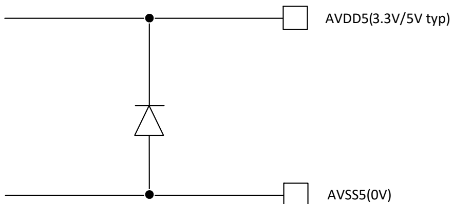
Figure 26. ESD Diodes between AVDD5 and AVSS5
