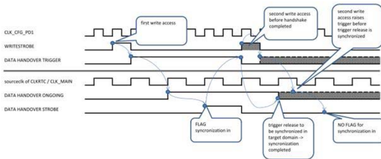
Figure 29. Handshake Synchronization
