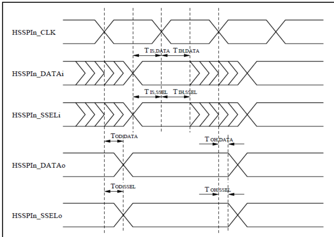
Figure 13. HSSPI Interface Timing
