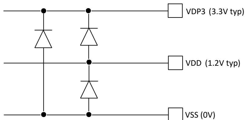
Figure 23. ESD Diodes between VDP3, VDD and VSS
