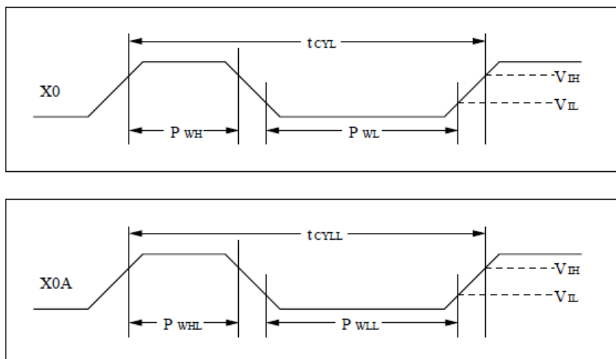
Figure 7. Source Clock Timing
