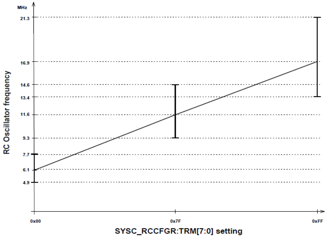
Figure 22. RC Oscillator Frequency at SYSC_RCCFGR:SFREQ = 1
