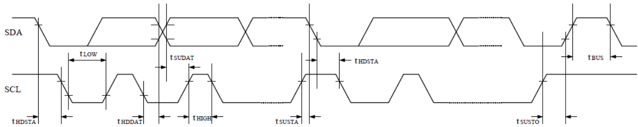
Figure 12. I2C Timing
