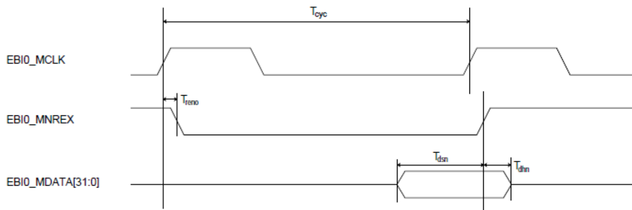
Figure 18. NAND Flash Read Timing
