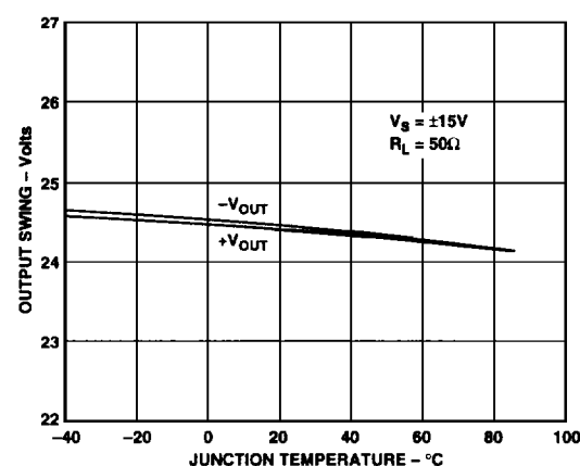
Figure 24. Differential Output Swing vs. Temperature
