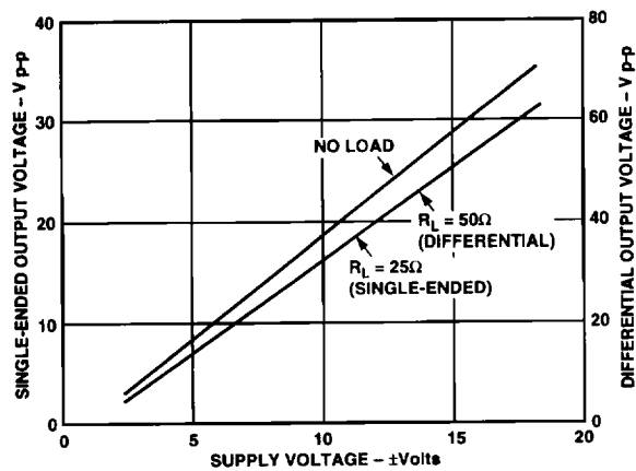
Figure 2. Output Voltage Swing vs. Supply Voltage
