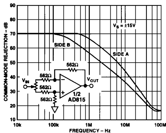
Figure 14. Common-Mode Rejection vs. Frequency
