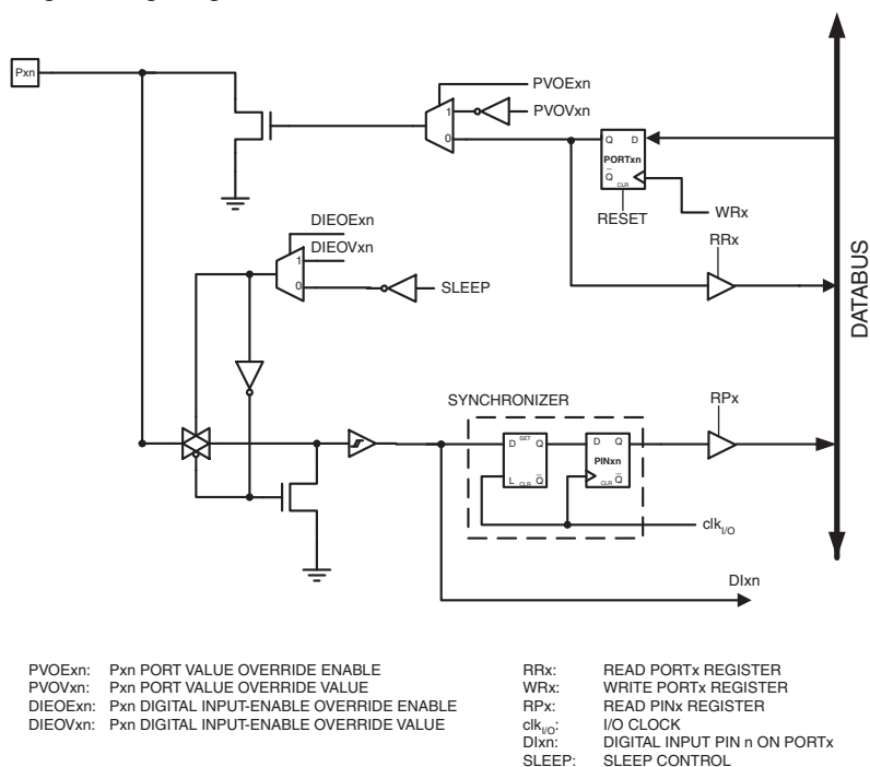
Figure 14-3. High voltage digital I/O (1)(2) .
