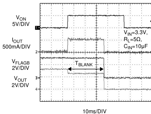
Figure 16. T BLANK Response
