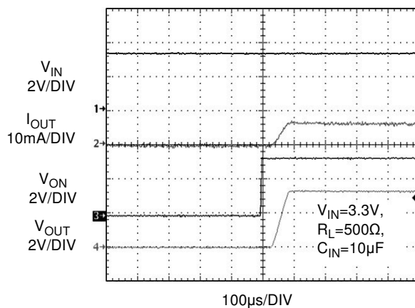
Figure 14. T ON Response
