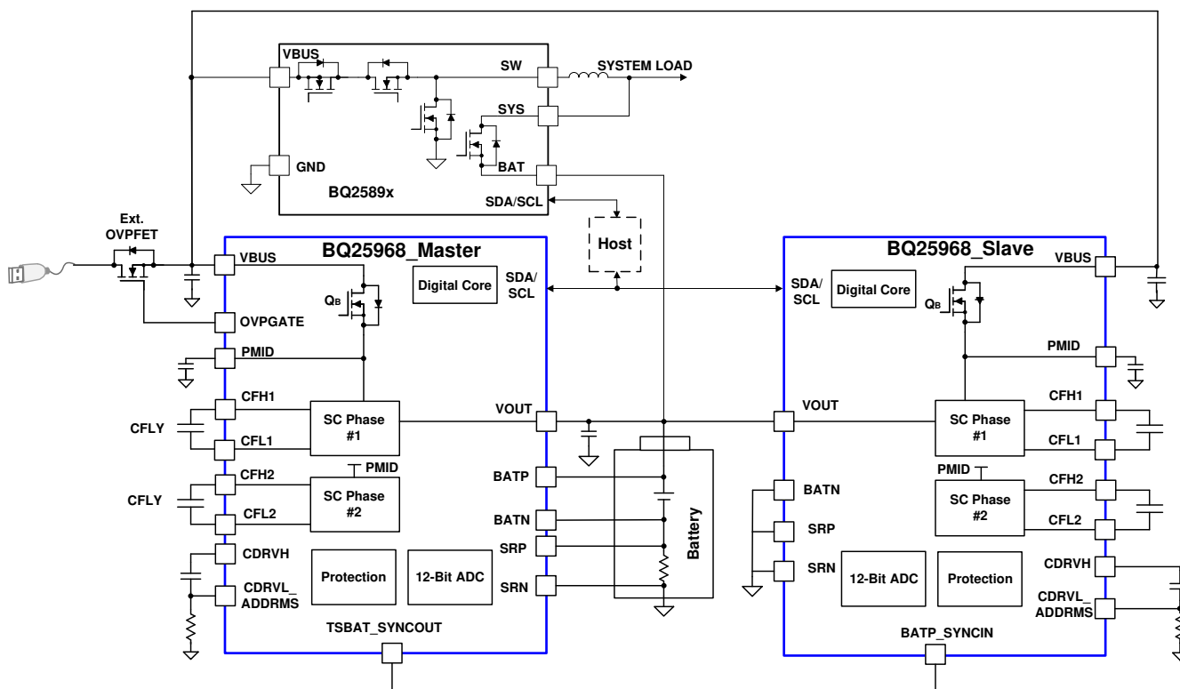
Figure 10-8. Parallel BQ25968 System
