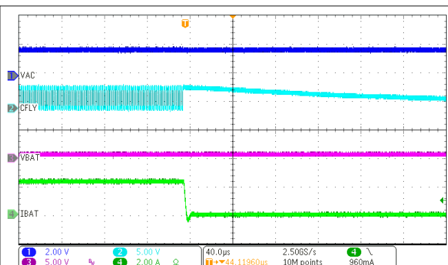
Figure 10-3. Disable Charge
