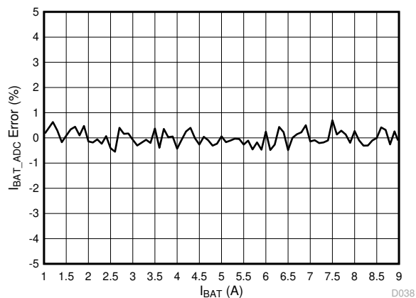
Figure 8-14. IBAT_ADC Error
