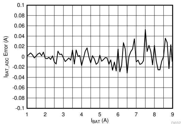
Figure 8-13. IBAT_ADC Error
