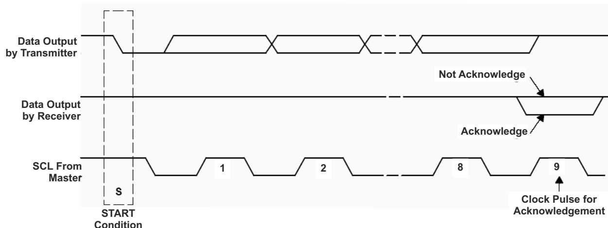
Figure 9-11. Acknowledge on the I²C BUS
