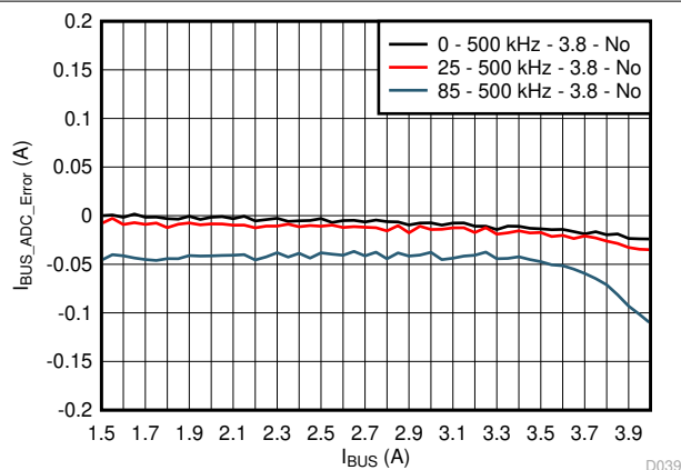
Figure 8-12. IBUS_ADC Error
