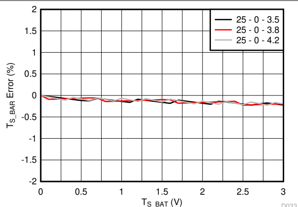
Figure 8-11. TS_BAT Error
