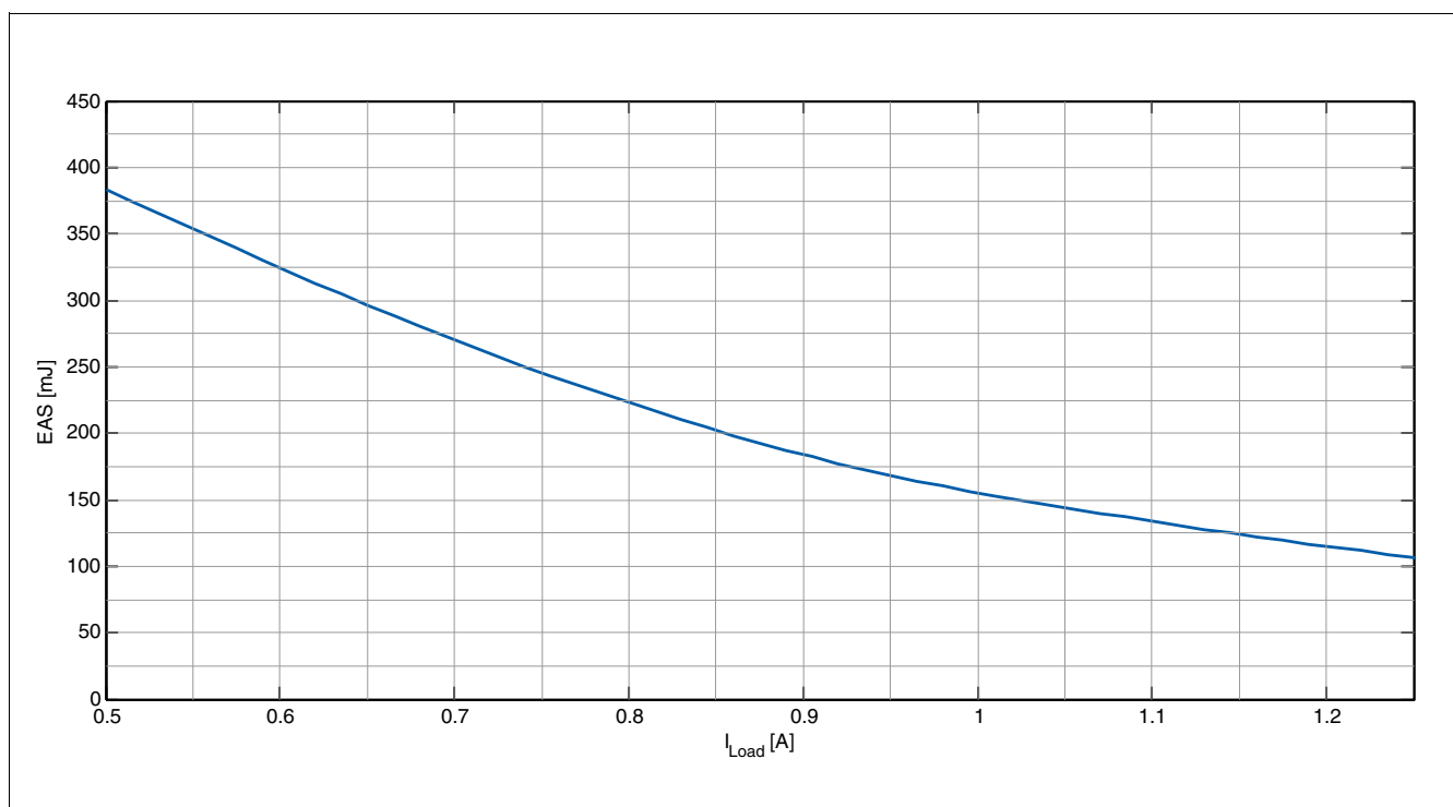
Figure 10 Maximum Energy Dissipation Single Pulse for a Single Channel ( T_j = 150^\circ C , V_S = 28 V )
