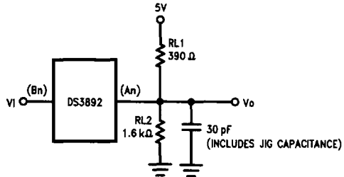
FIGURE 2. Receiver Propagation Delays
