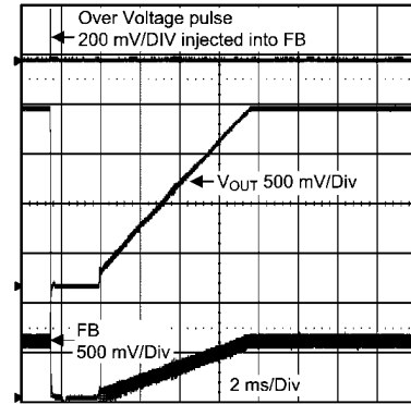
Over-Voltage Fault
