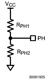
FIGURE 5. Phase Selection
