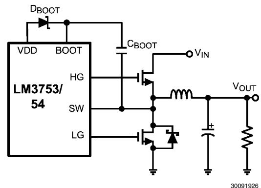
FIGURE 6. Bootstrap Circuit
