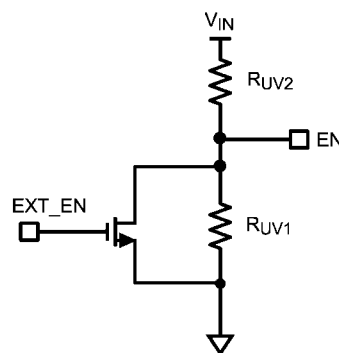
FIGURE 4. Input Voltage UVLO with External Enable
