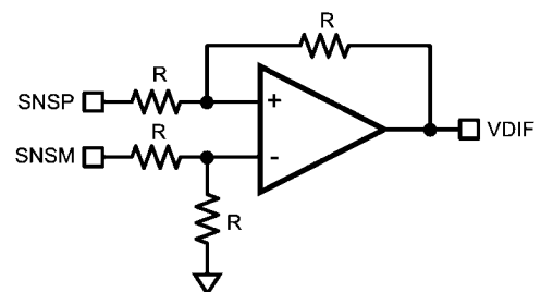
FIGURE 7. Differential Amplifier
