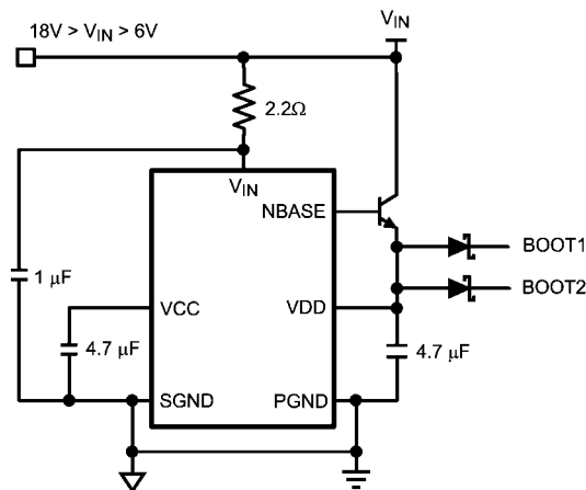
FIGURE 1. Power Connections Using the Internal Regulator
