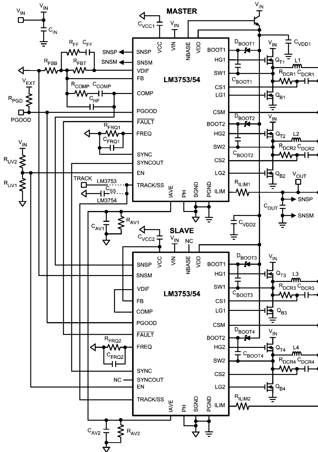
FIGURE 20. Typical Application
