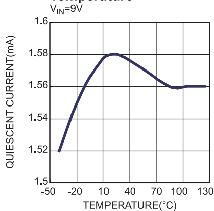
Quiescent Current vs. Temperature V_{IN}=9V
