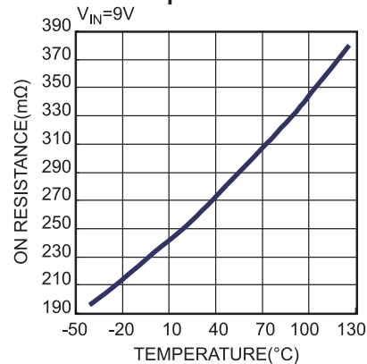
Bridge A HS On Resistance vs. Temperature V_{IN}=9V
