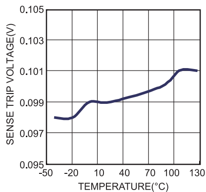
50% Sense Trip Voltage vs. Temperature
