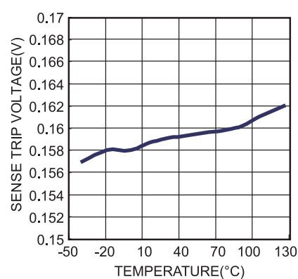
80% Sense Trip Voltage vs. Temperature
