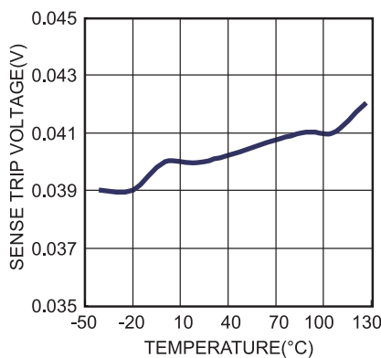
20% Sense Trip Voltage vs. Temperature
