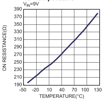
Bridge B HS On Resistance vs. Temperature V_{IN}=9V
