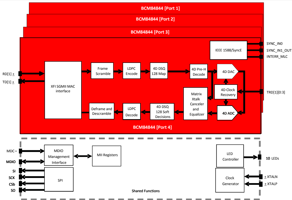
BCM84844 Block Diagram for Each Port
