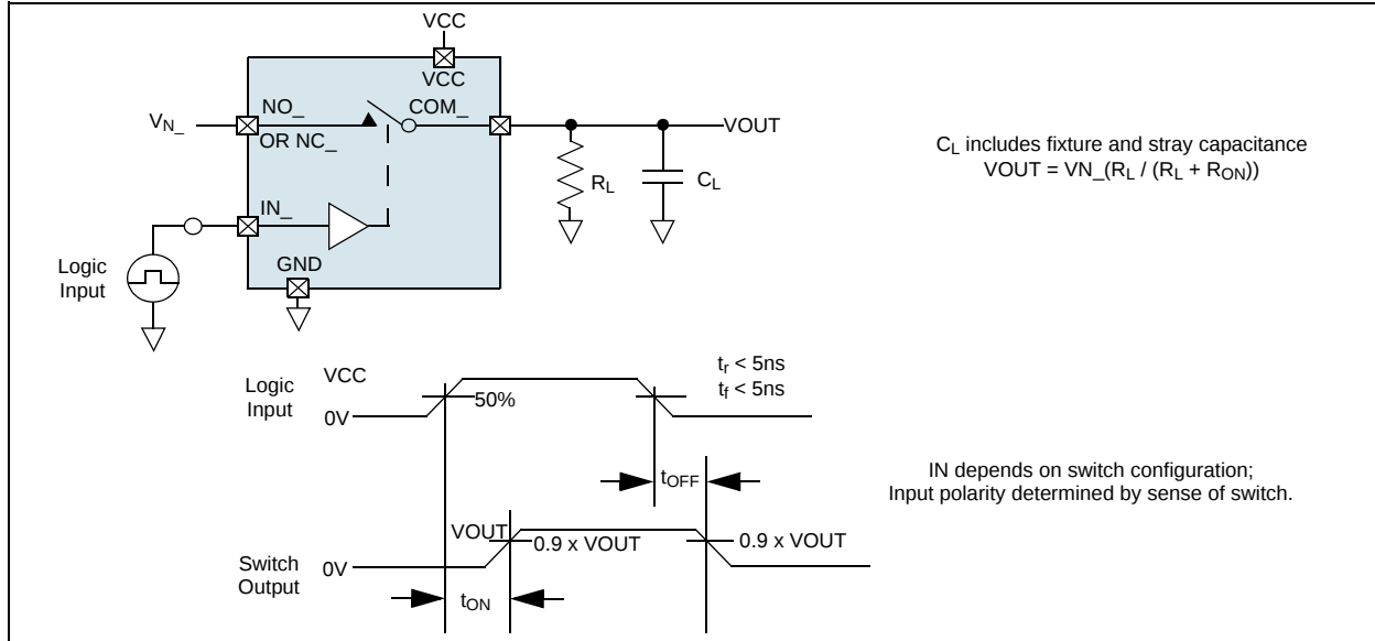
Figure 19. Switching Time
