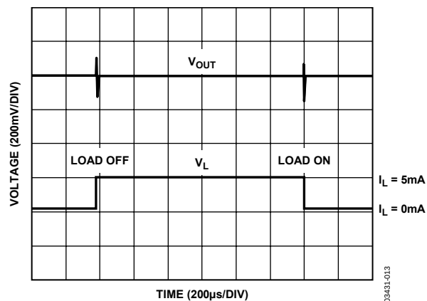
Figure 13. Load Transient Response, C_L = 100 nF
