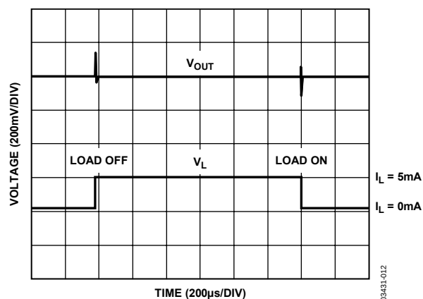
Figure 12. Load Transient Response, C_L = 1 nF
