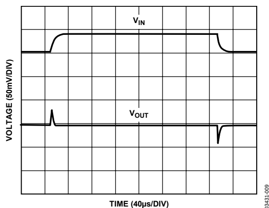
Figure 9. Line Transient Response, C_{BYPASS} = 0 \mu F
