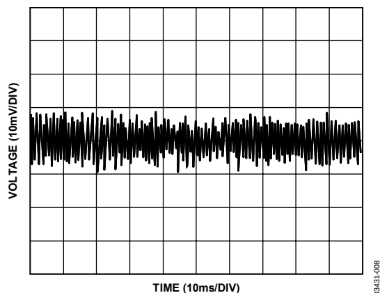
Figure 8. Typical Output Voltage Noise 10 Hz to 10 kHz
