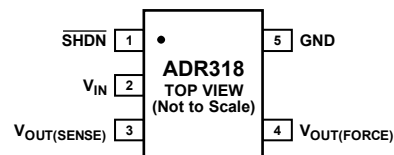
Figure 1. 5-Lead SOT-23
