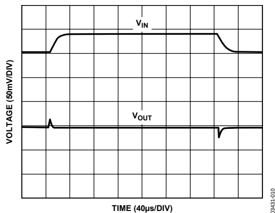
Figure 10. Line Transient Response, C_{BYPASS} = 0.1 \mu F
