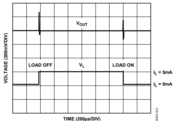
Figure 11. Load Transient Response, C_L = 0 nF
