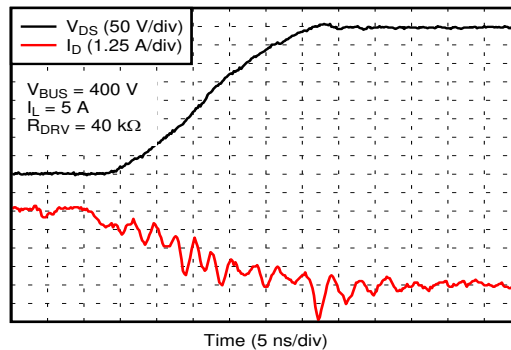
Figure 10-4. Turn-Off Waveform in Application Example
