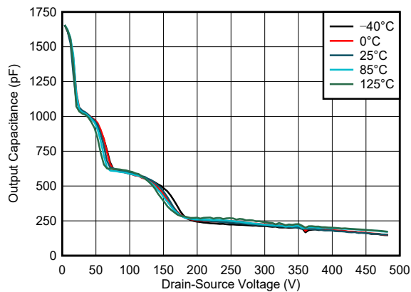
Figure 7-9. Output Capacitance vs Drain-Source Voltage
