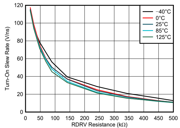
Figure 7-4. Turn-On Slew Rate vs Drive Strength Resistance
