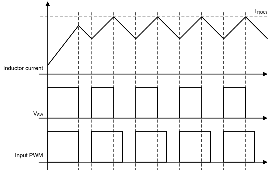
Figure 9-2. Cycle-by-Cycle OCP Operation
