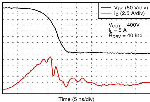
Figure 10-3. Turn-On Waveform in Application Example
