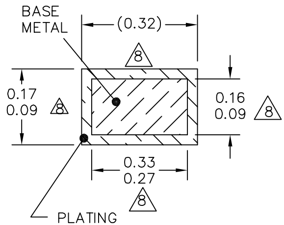
SECTION B-B
