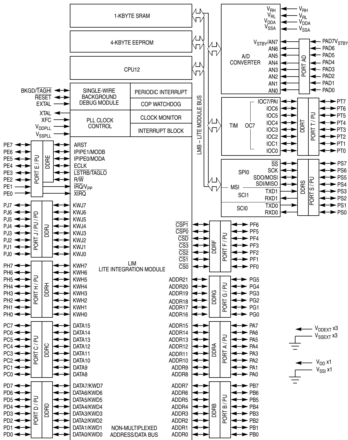
Figure 1-2. Block Diagram
