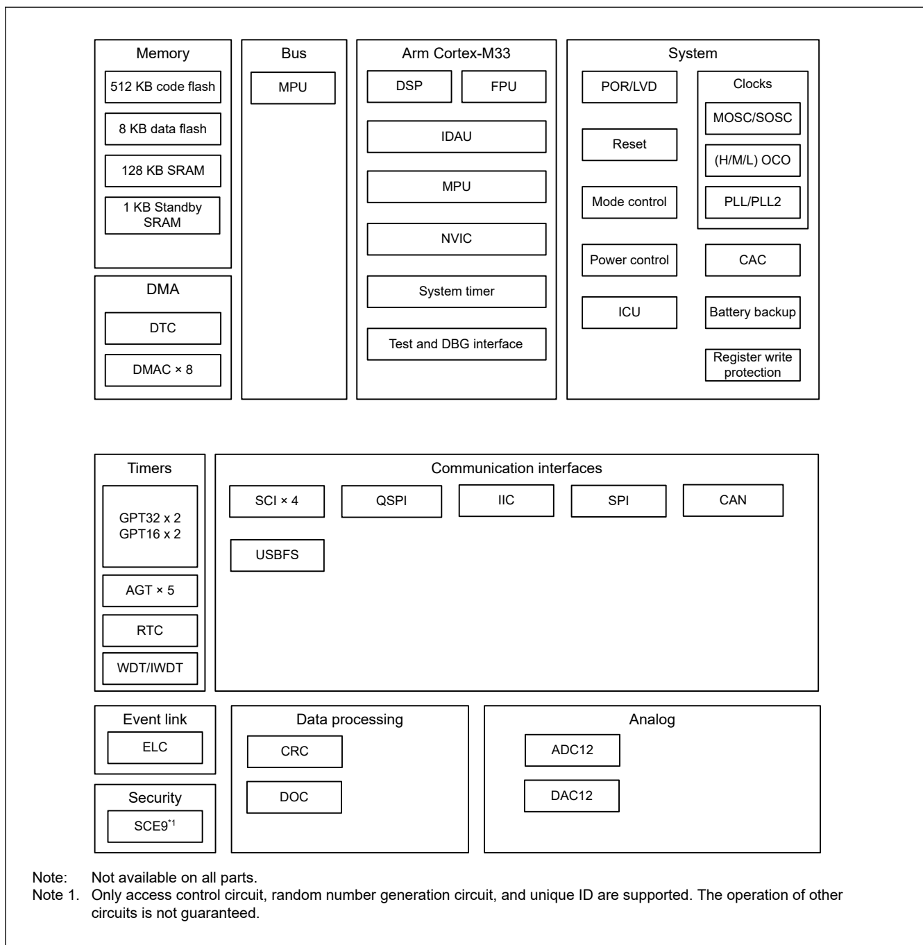
Figure 1.1 Block diagram
