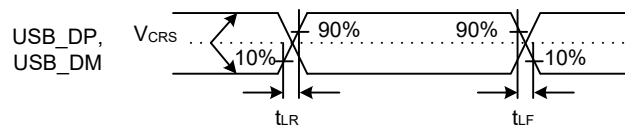
Figure 2.43 USB_DP and USB_DM output timing in low-speed mode
