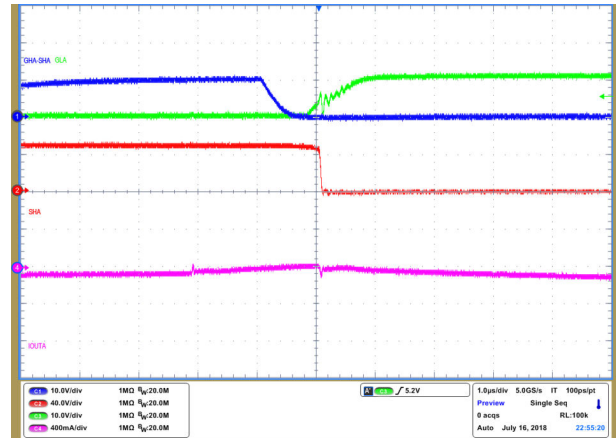
Figure 14-5. IDrive Minimum Setting Negative Current
