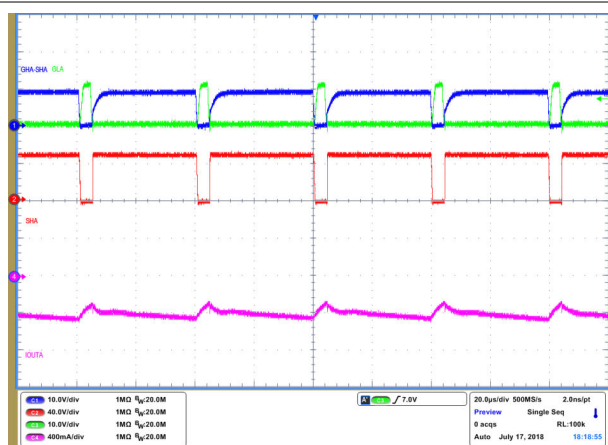
Figure 14-3. Gate Driver Operation 90% Duty Cycle
