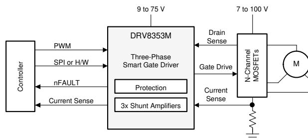
Simplified Schematic
