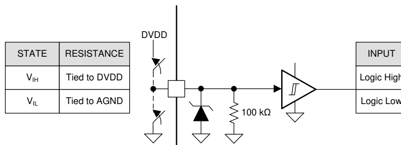
Figure 13-17. Logic-Level Input Pin Structure
