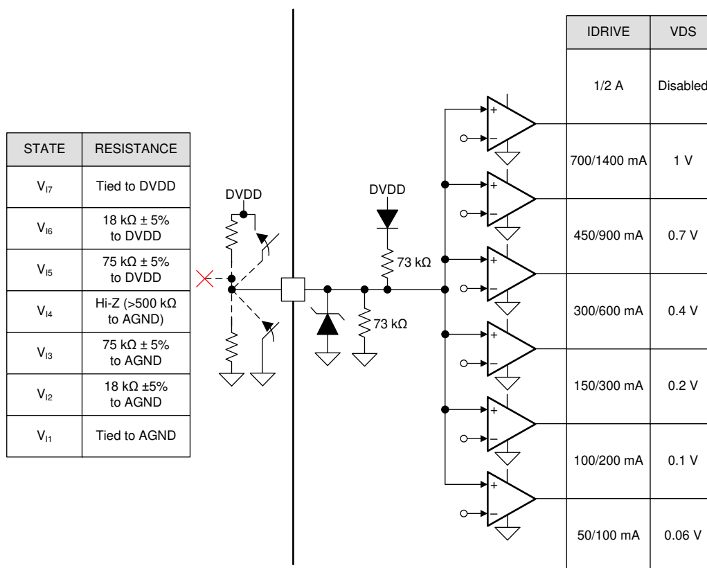
Figure 13-19. Seven Level Input Pin Structure
