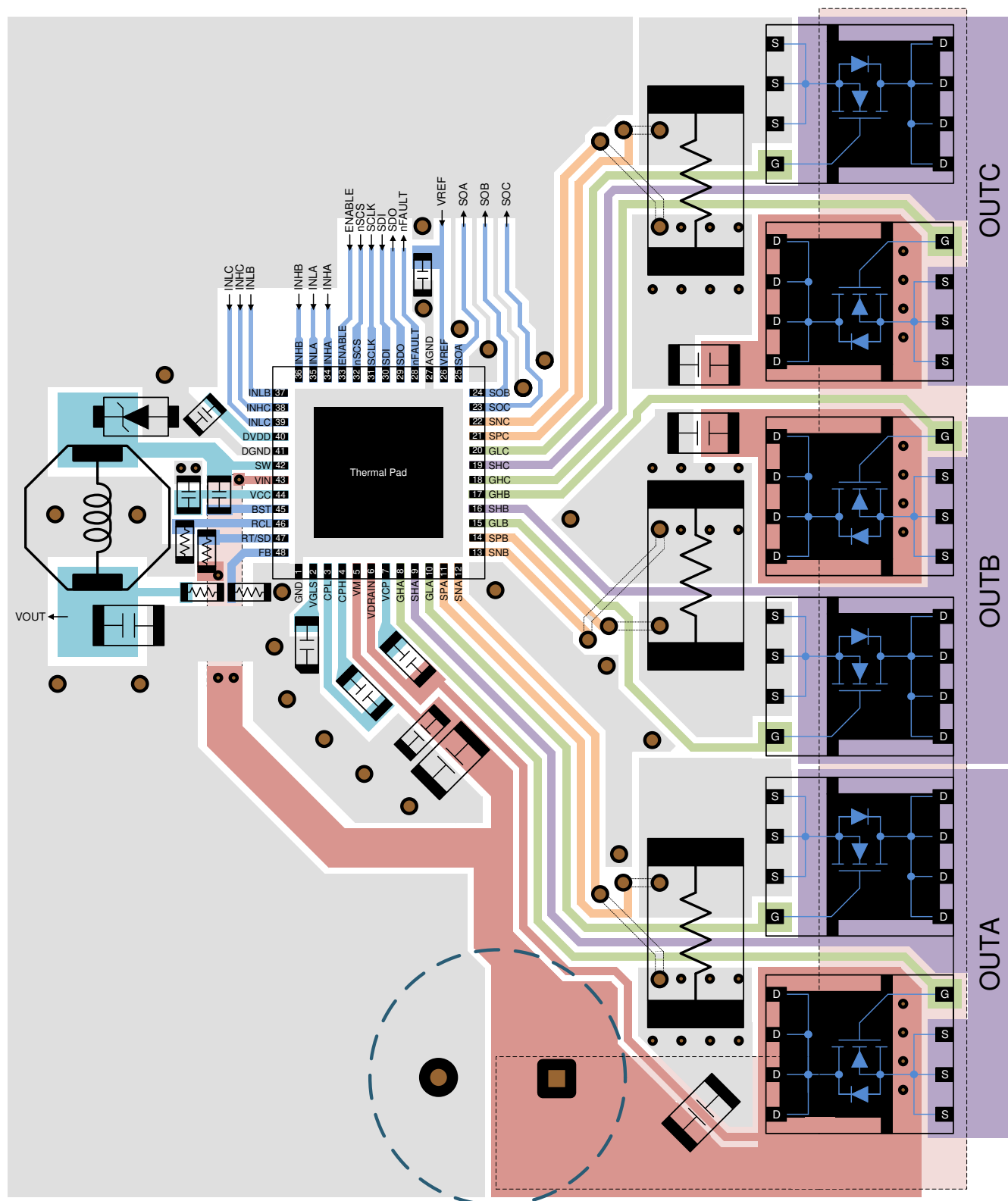
Figure 16-1. Layout Example
