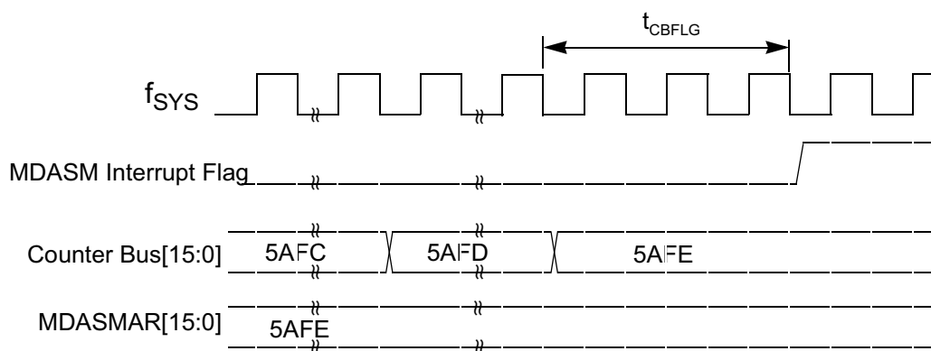
Figure G-49 Counter Bus to MDASM Interrupt Flag Setting Timing Diagram
