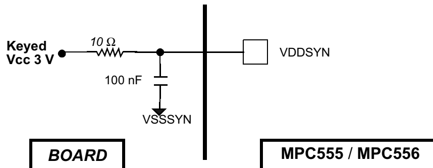
Figure E-6 RC Filter Example
