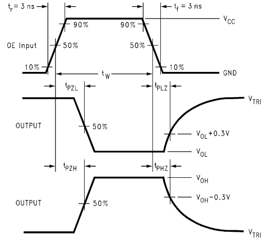
Figure 6. AC Waveforms
