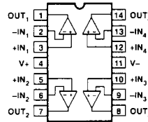
14-PIN HERMETIC DIP (Y-Suffix)
