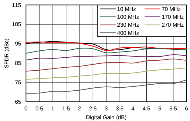
Figure 86. SFDR vs Digital Gain and Input Frequency
